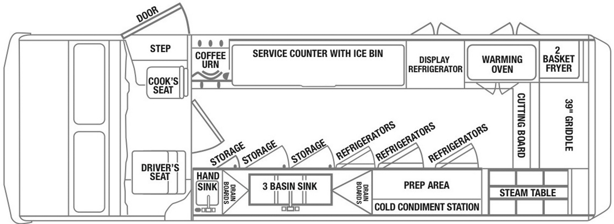
Route Truck Dimensions: 11' H x 24.4' L x 7.3' W, 13' wheel base
